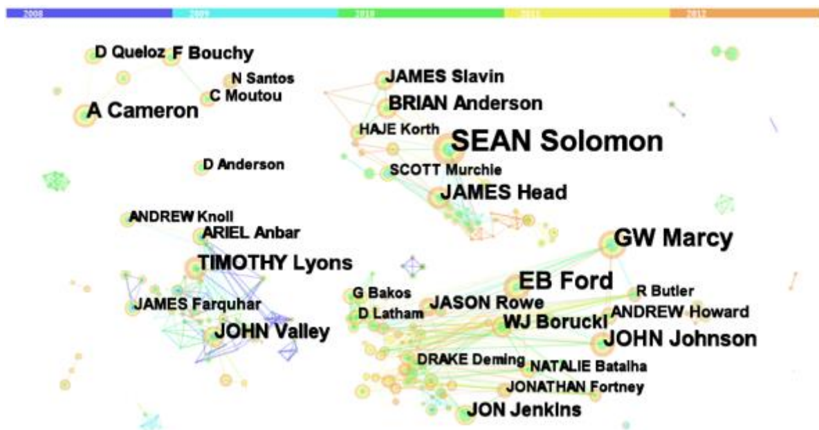
Figure 7: Co-authorship clusters
